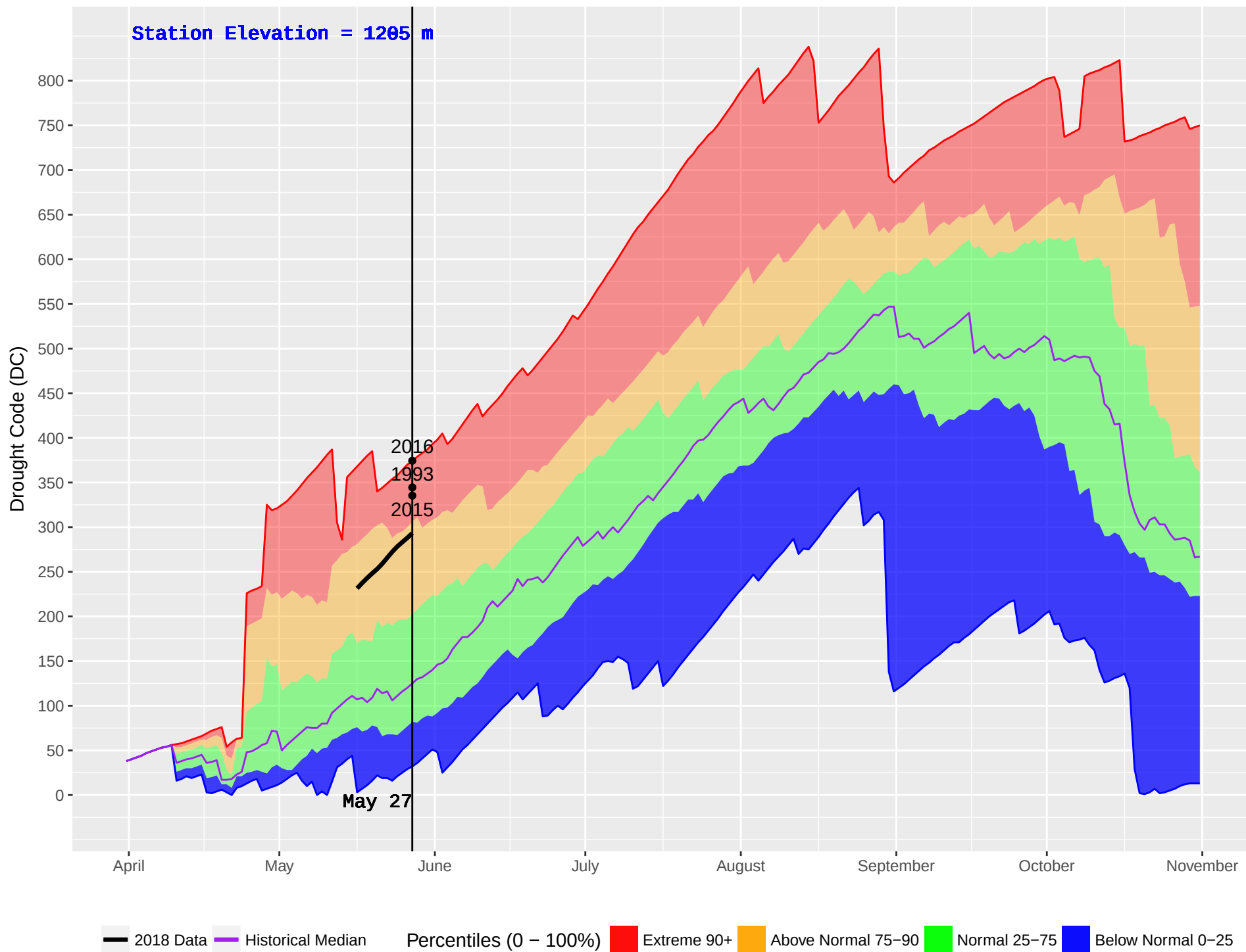
GWYNETH LAKE (309) : Historical (1986–2016) and Current (2018) Noon Drought Code (DC)
