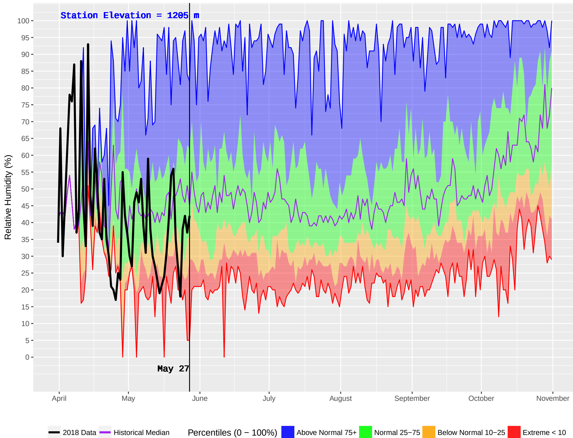
GWYNETH LAKE (309) : Historical (1986–2016) and Current (2018) Noon Relative Humidity
