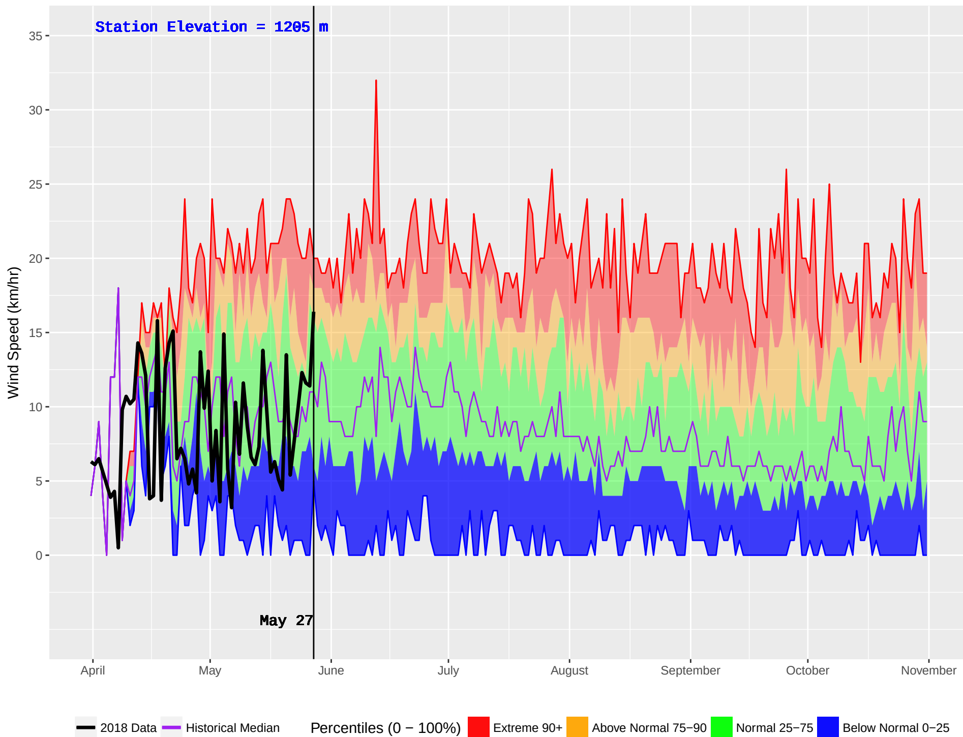
GWYNETH LAKE (309) : Historical (1986–2016) and Current (2018) Noon Wind Speed
