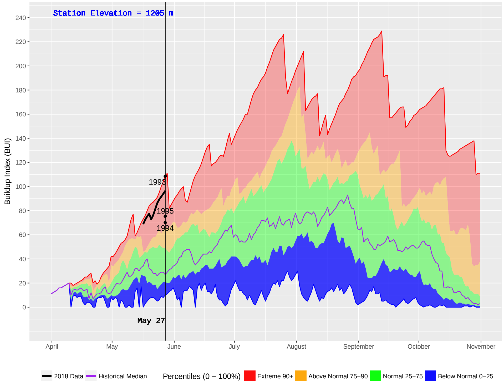
GWYNETH LAKE (309) : Historical (1986–2016) and Current (2018) Noon Buildup Index (BUI)
