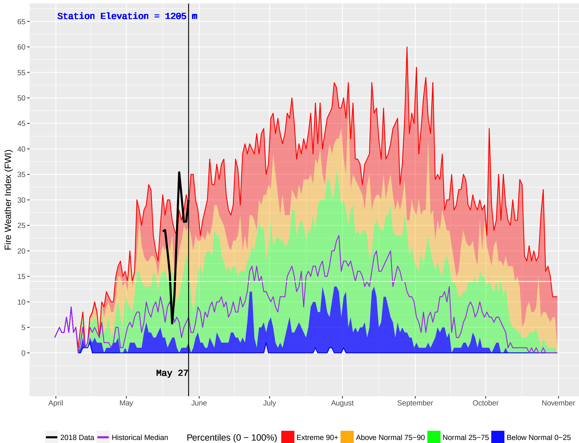
GWYNETH LAKE (309) : Historical (1986–2016) and Current (2018) Noon Fire Weather Index (FWI)
