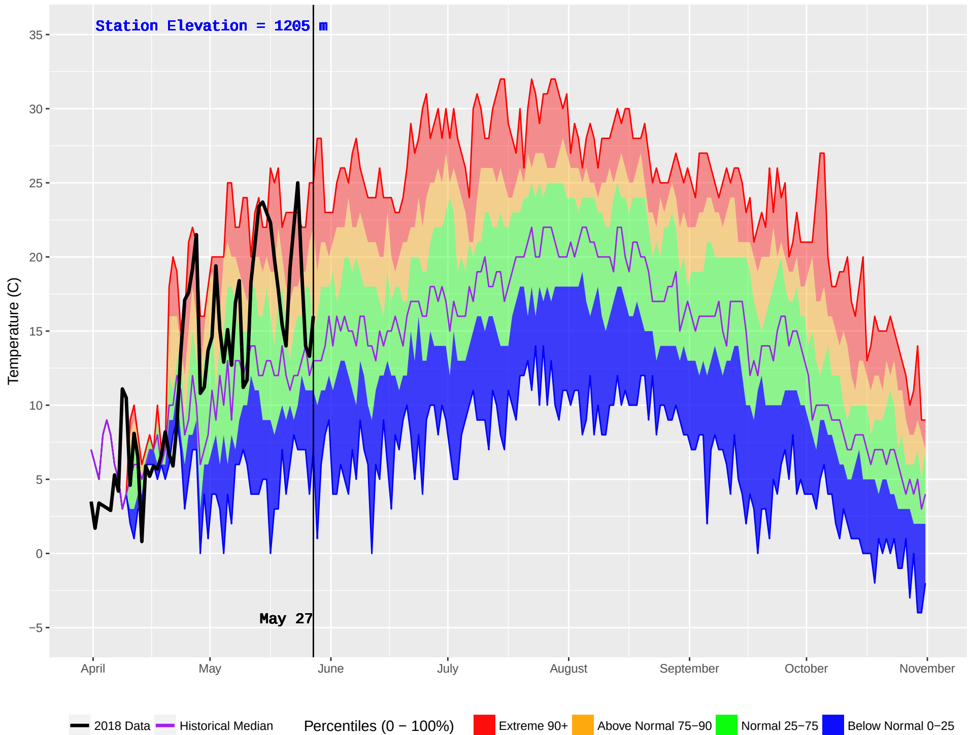
GWYNETH LAKE (309) : Historical (1986–2016) and Current (2018) Noon Temperature
