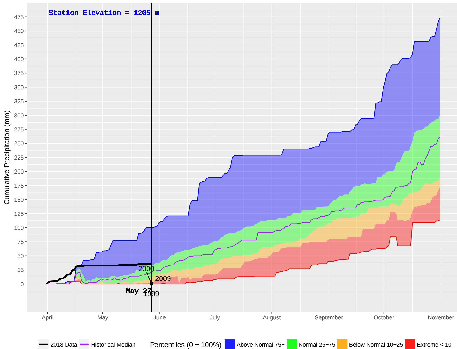
GWYNETH LAKE (309) : Historical (1986–2016) and Current (2018) Noon Cumulative Precipitation
